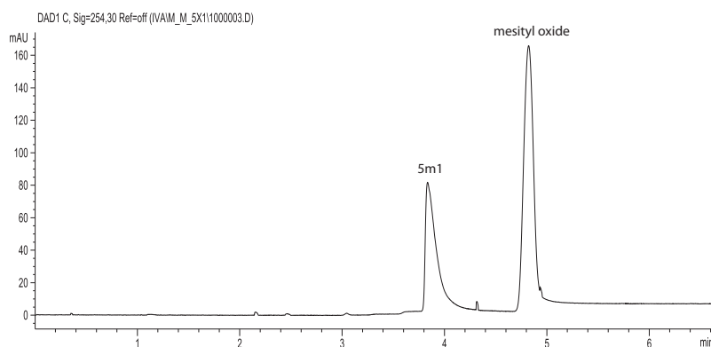
Fig. 1. Electropherogram of compound 5m1 ( 7.5 \cdot 10^{-4} \text{ mol.l}^{-1} ) and mesityl oxide ( 2 \cdot 10^{-6} \text{ mol.l}^{-1} ) in MOPSO/NaOH background electrolyte ( \text{pH} = 6.70 , I = 0.01 \text{ mol.l}^{-1} ), injection by pressure 40 mbar for 4 s, applied voltage +15 kV, temperature 25^\circ\text{C} , detection at 254 nm
