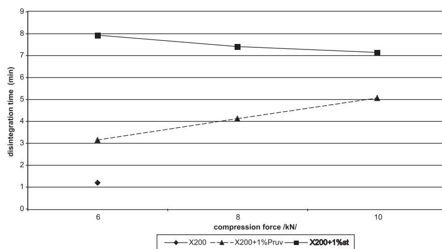
Fig. 5. Disintegration time in function of compression force: Xylitab 200 with lubricants
