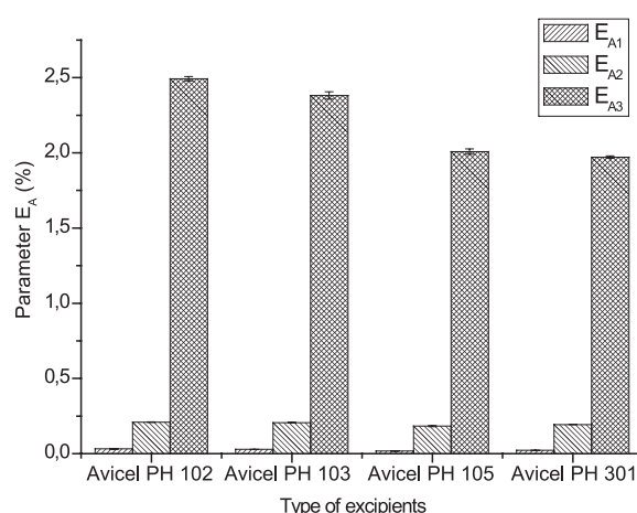
Fig. 4. Parameters E_{A1-3} in the excipients under study (all columns displayed means of n = 20 with 1s error bars)
