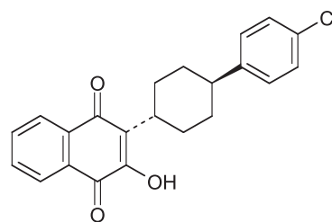
Obr. 4. Atovaquon – trans-2-[4-(4-chlorfenyl)-cyklohexyl]-3-hydroxy-1,4-naftochinon, C 22 H 19 ClO 3
